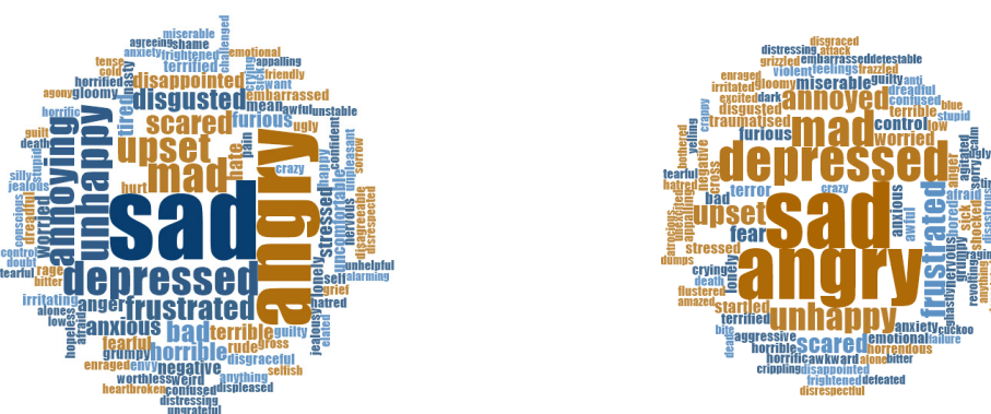
Figure 3. Student unpleasant high energy emotion vocabulary pre- (left) and post- (right) results.
